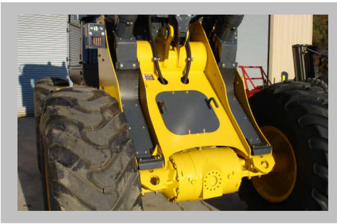
Boom Cylinder Cavity Guards
